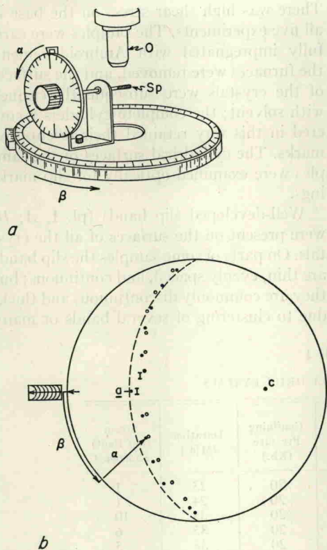
FIG. 1.— a , apparatus for measuring orientation of slip bands on surface of polished cylinders. Microscope objective ( O ) and specimen ( Sp. ) are indicated. Angles \alpha and \beta are the angles of rotation of the graduated circle and microscope stage, respectively. b , equal-area projection showing orientation of slip bands on crystal C-247, along with crystal showing orientation mark (arrow) and slip bands. Original crystallographic orientation of sample is shown by c - and a -axes in the projection. Broken line is the original orientation of basal plane; open circles and black circles represent orientations of slip bands measured on back and front of the cylinder, respectively, and short line segments represent null zones on each side of the cylinder.
